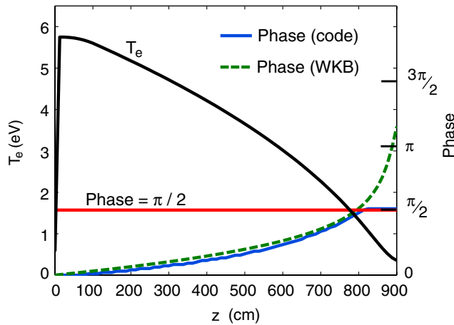
FIG. 3 (color online). Axial dependence of resonator. Curve labeled T_e is the steady-state axial temperature profile predicted by transport code. Solid blue curve is the axial phase of a temperature wave at 5.1 kHz also obtained from the code. Dashed green line is a WKB phase calculation using the dispersion relation of Eq. (1). Red line corresponds to a wave phase of \pi/2 . Intercept of curves shows system behaves as a quarter-wave thermal resonator.
