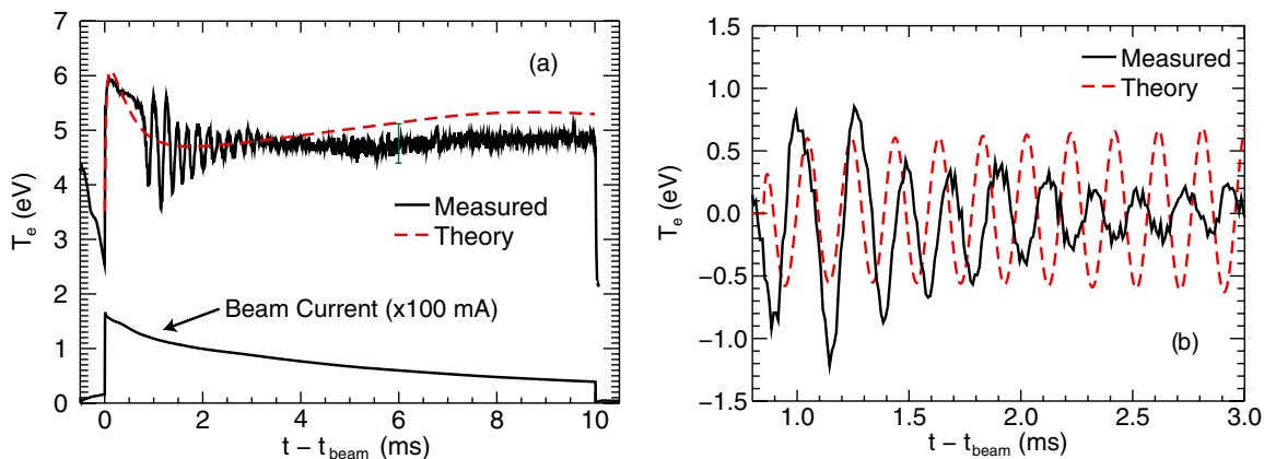
FIG. 1 (color online). Time evolution of electron temperature, T_e , at a position 224 cm axially away from the beam source at the filament center. (a) Development over the full beam-pulse. (b) The spontaneous coherent thermal oscillation over a 2.2 ms interval. Solid curves are experimental measurements and dashed curves are predictions of the transport code. The code result in (a) does not include a driven thermal wave, while in (b) a modulation at 5.1 kHz is included. The bottom trace in (a) is the injected beam current.
