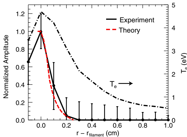
FIG. 2 (color online). Solid curve shows the radial dependence of the normalized amplitude of the coherent thermal oscillations at z = 544 cm. Dashed curve is the prediction of the transport code. The top dashed-dotted curve is the radial profile of the electron temperature filament.
